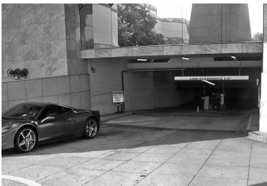
▲ Foxwoods Resort Casino, Mashantucket, Connecticut, Grand Pequot Parking Garage Assessment and Repair.
