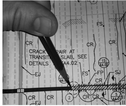
Drawings are useful for marking locations of distress, past repairs, and other conditions.
