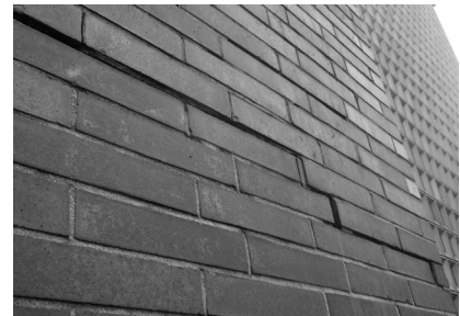
▲ Lateral displacement of brick veneer.
