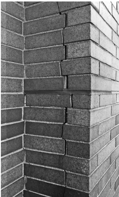
▲ Long, vertical cracks at building corners may indicate underlying structural distress.
