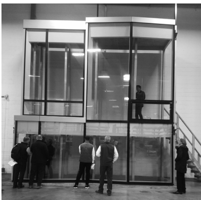
▲ Mockups verify aesthetics and performance.
