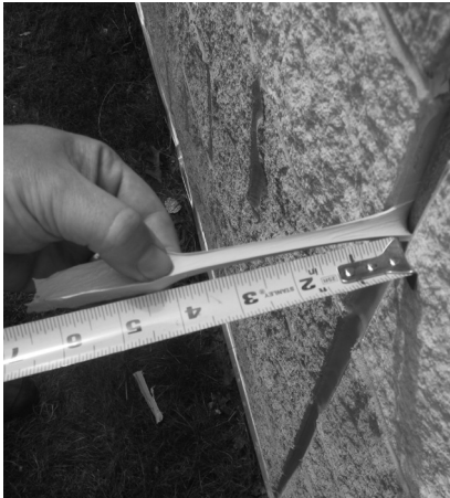
▲ Peel tests are used to evaluate sealant elongation and adhesion.
