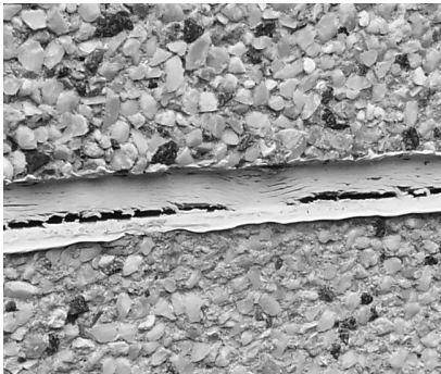
▲ Cohesive failure: Sealant tears within itself.
