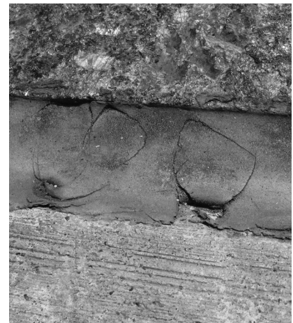
▲ Damage to plaza sealant caused by high heels.
