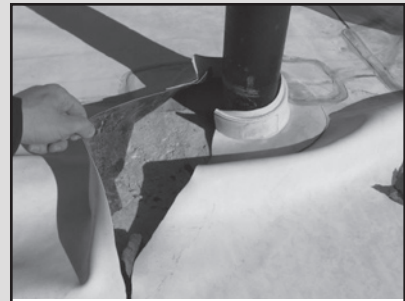
▲ Poor anchorage and weak membrane adhesion were signs that this roof failure could have been avoided.
