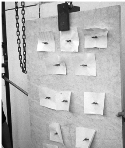
▲ Replacement panel mock-up to assess anchor geometry and installation protocol.
