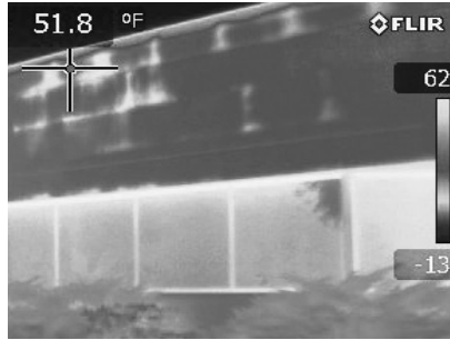
A This infrared thermographic scan reveals trapped moisture at insulation board joints.
