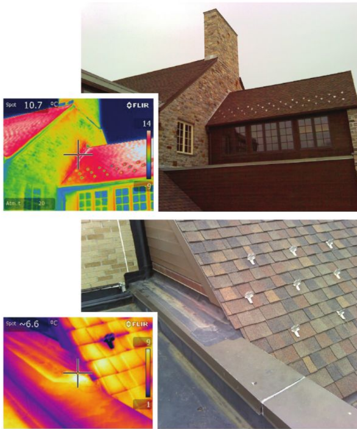
Infrared thermography photographs highlight areas of heat loss with color hues that represent thermal gradients.
